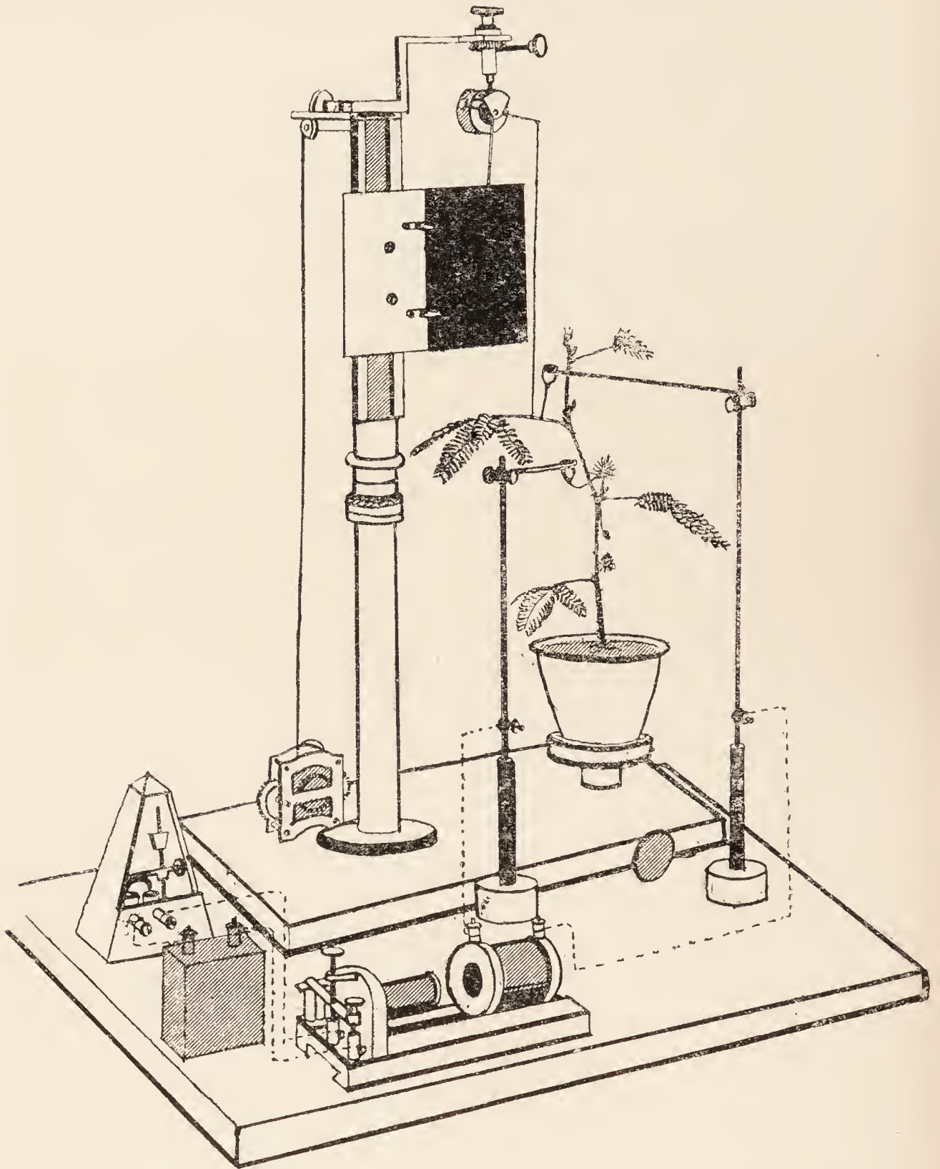
FIG. II.—General view of the Resonant Recorder and the electrical connections by which excitatory shock of a definite duration is given to the plant; duration of shock determined by metronome, which completes electric circuit.
